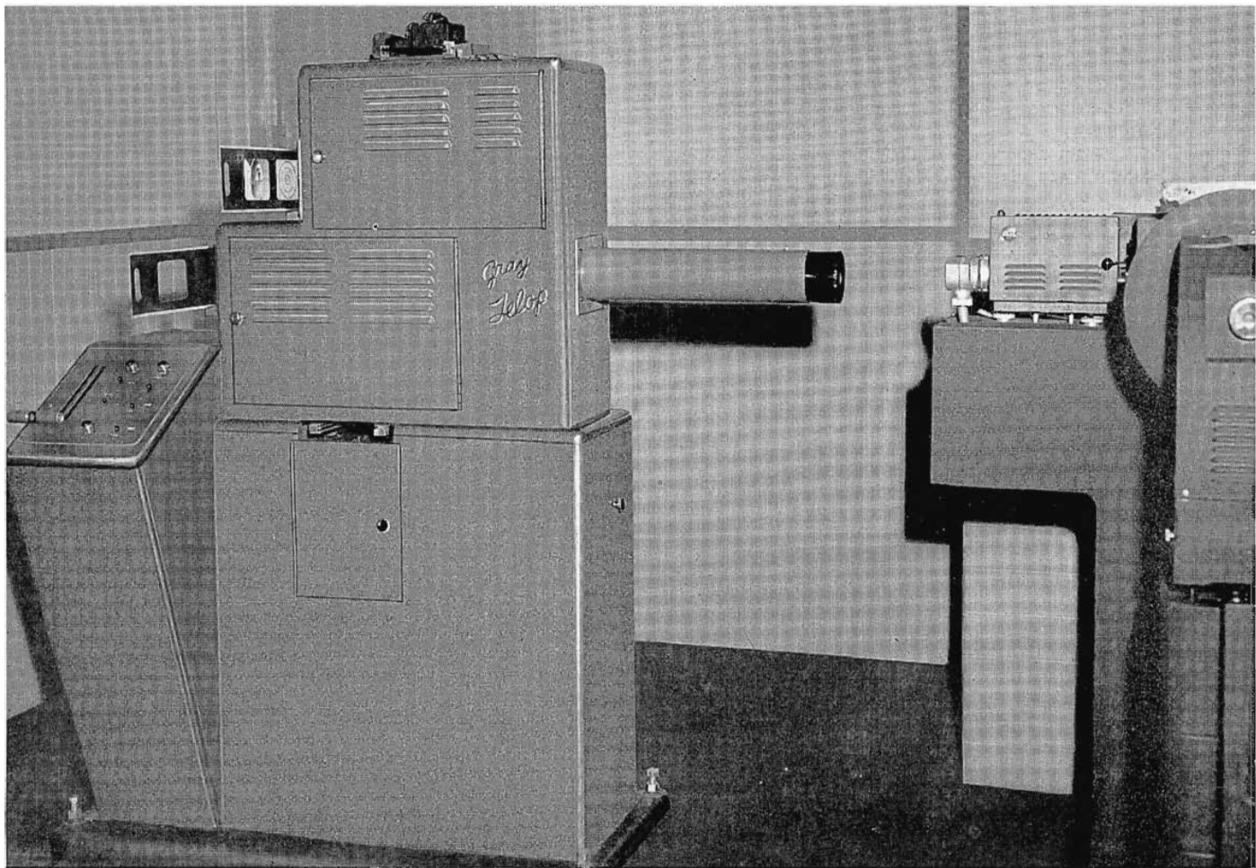
A Telop I, formerly used with one of the iconoscope chains, is directed into one of the TP-11 Multiplexer inputs. In order to use the Telop with the TP-11, it was necessary to fabricate a new lens mount. Details of this revision can be found in the text.
