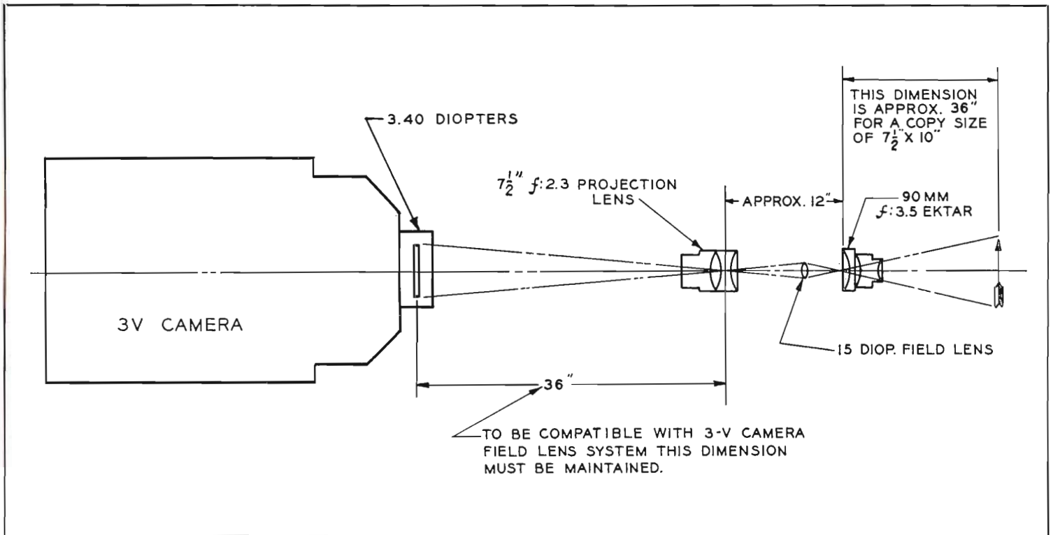
FIG. 2. Optical system showing lens arrangement for live commercial pickup. The Ektar lens is identical with those used on RCA image-orthicon cameras.
