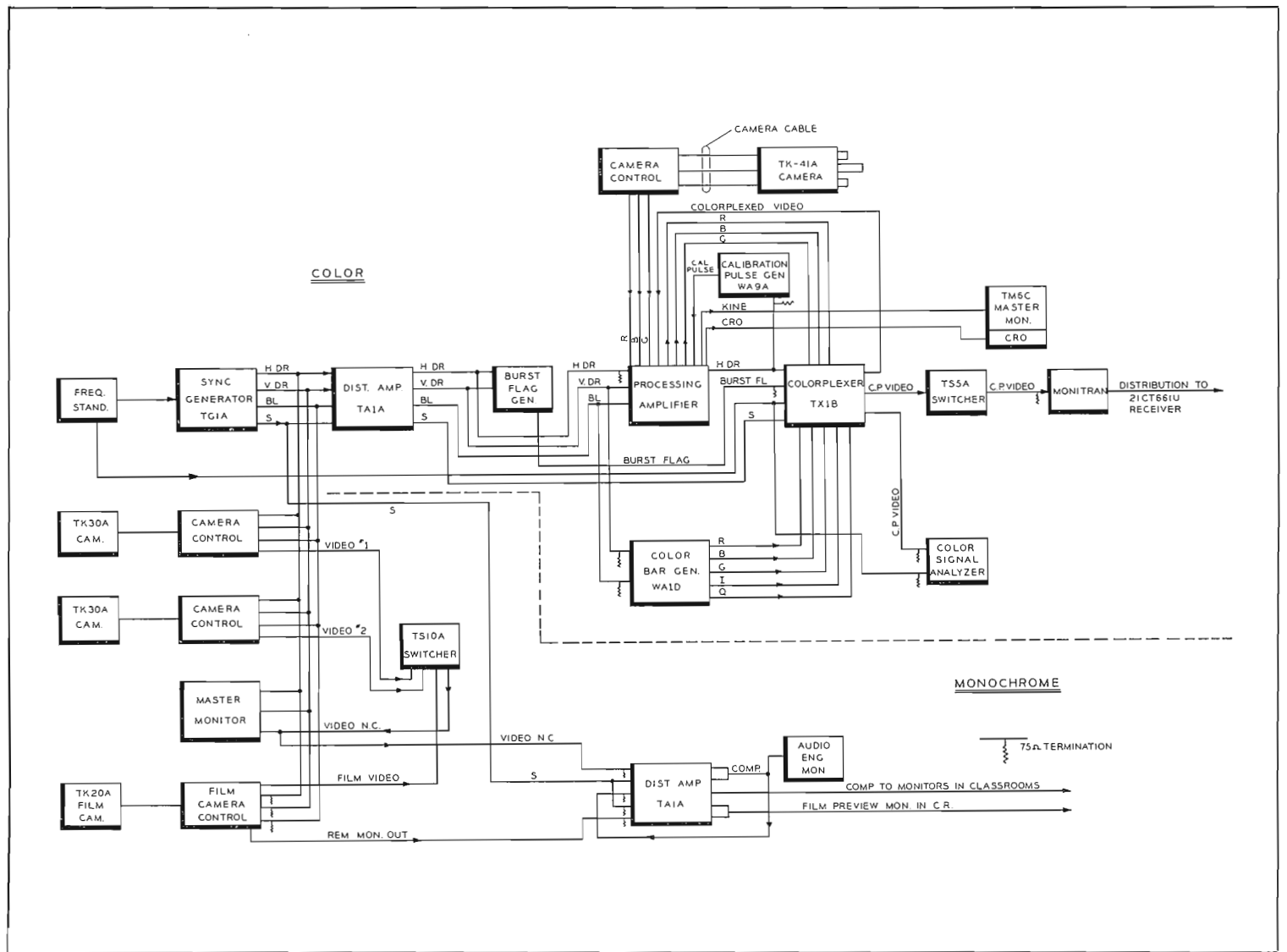
FIG. 4. Complete pulse and video distribution system at the SRT-TV Studios for closed circuit operations.
