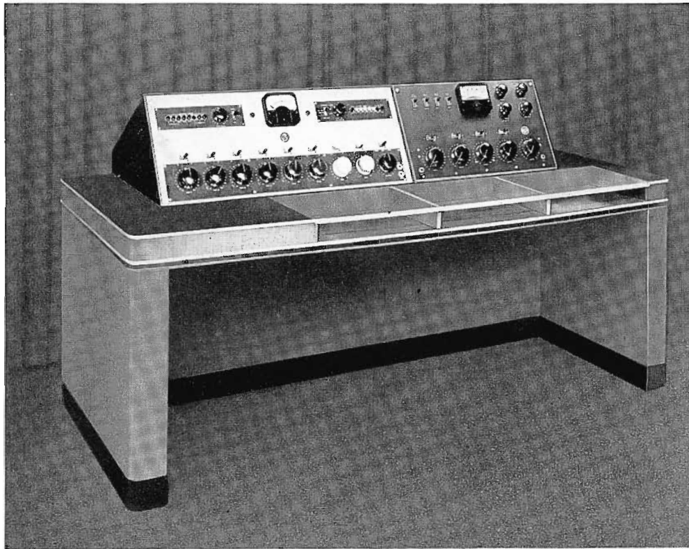
FIG. 5. The new BC-5A can be paired with existing BC-2B's by coupling the output of the BC-5A to a BC-2B microphone input position. The mixer associated with the BC-2B mike position becomes master control over the BC-5A.
