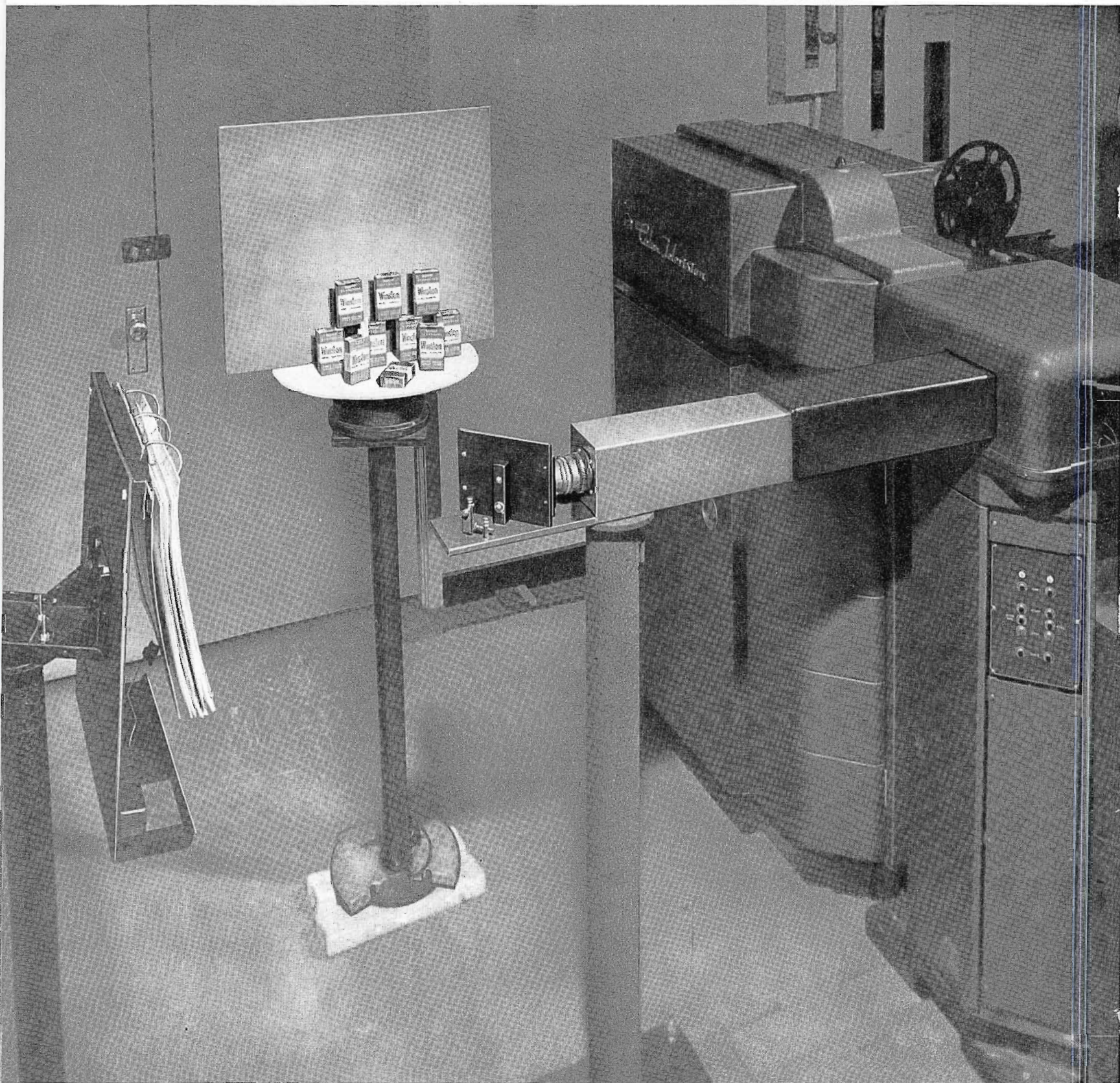
"3V" Color Film System as arranged for pickup of color opaques and live action commercials.
