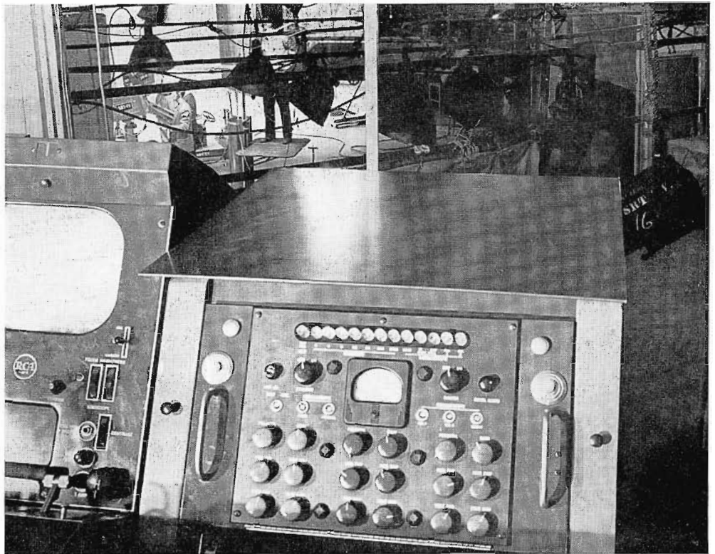
FIG. 5. View of the large TV studio from the color control room located at opposite end of studio from black and white control room. The Color Camera Control Panel is located to the left of Processing Amplifier.
