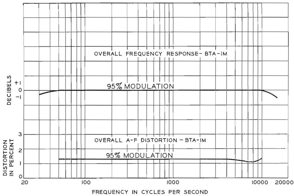
FIG. 9. Response curves show capability of high-fidelity performance from WDAS transmitter.
