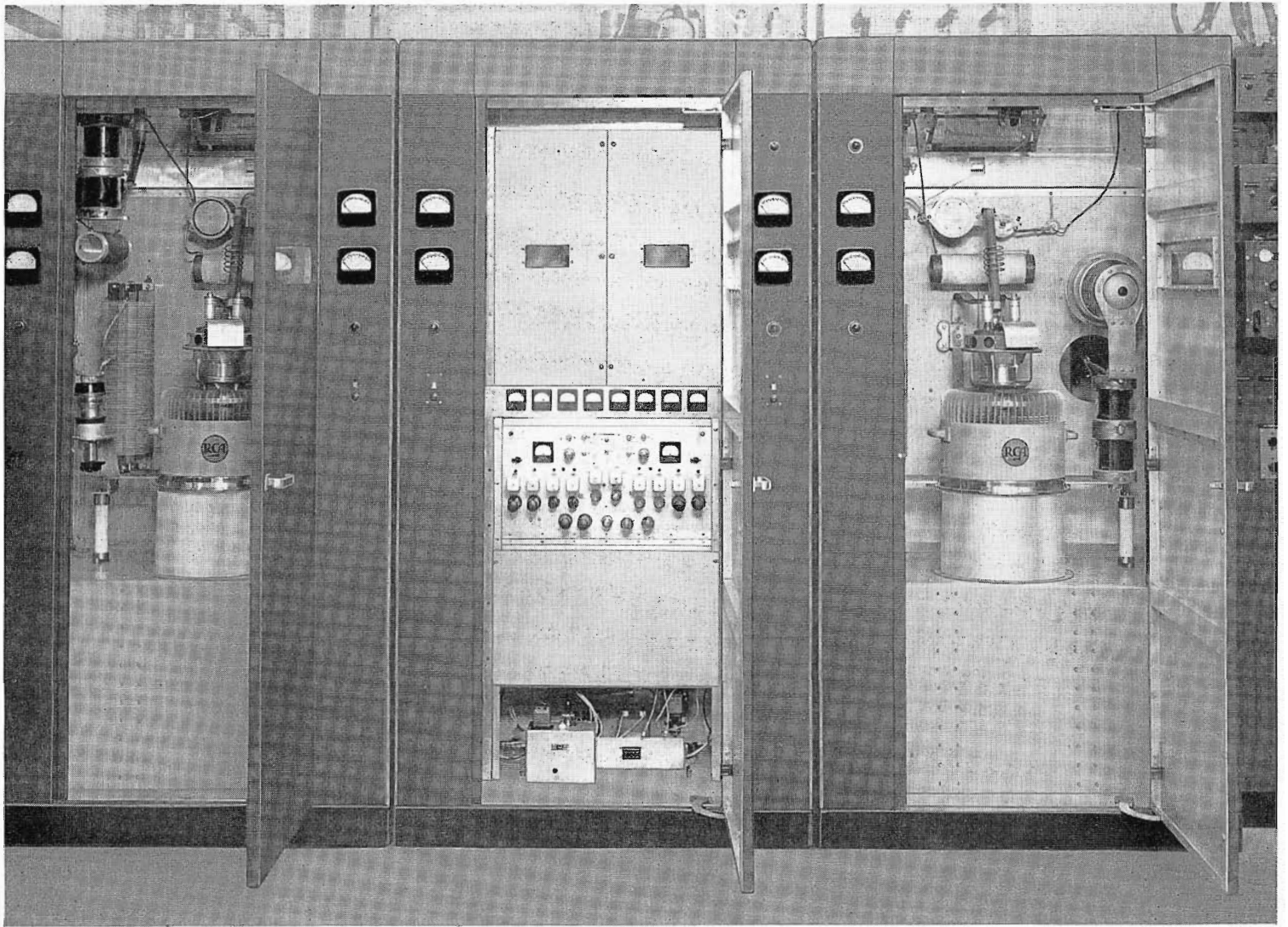
Part of new RCA type BTA-50G AM transmitter just prior to shipment to station WINS. Three of the four cubicles are shown—the two final power amplifier cubicles on either side of the exciter unit.
