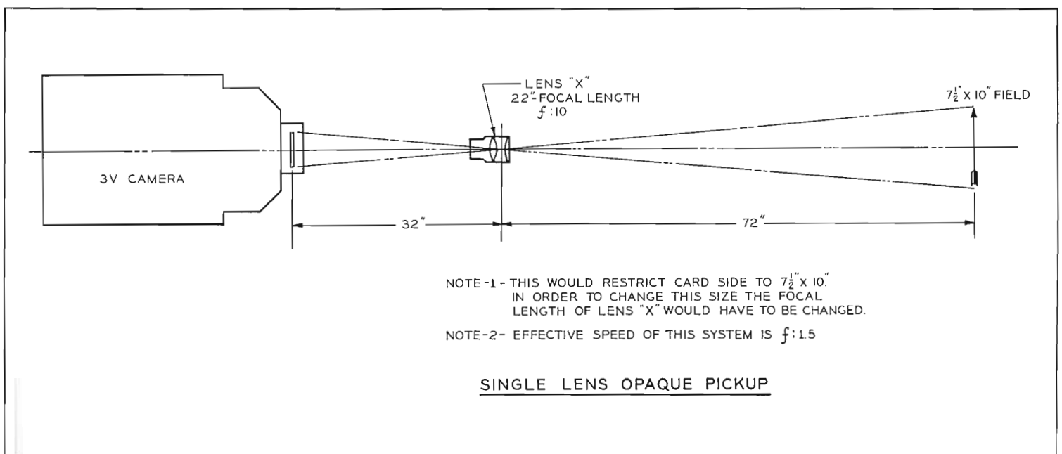
FIG. 3. Brute force optical approach demonstrates design flexibility of first lens arrangement shown in Fig. 2.
