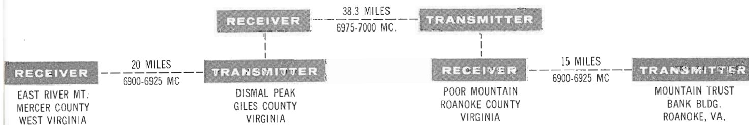
FIG. 5. Diagram of WHIS-TV Microwave system.
