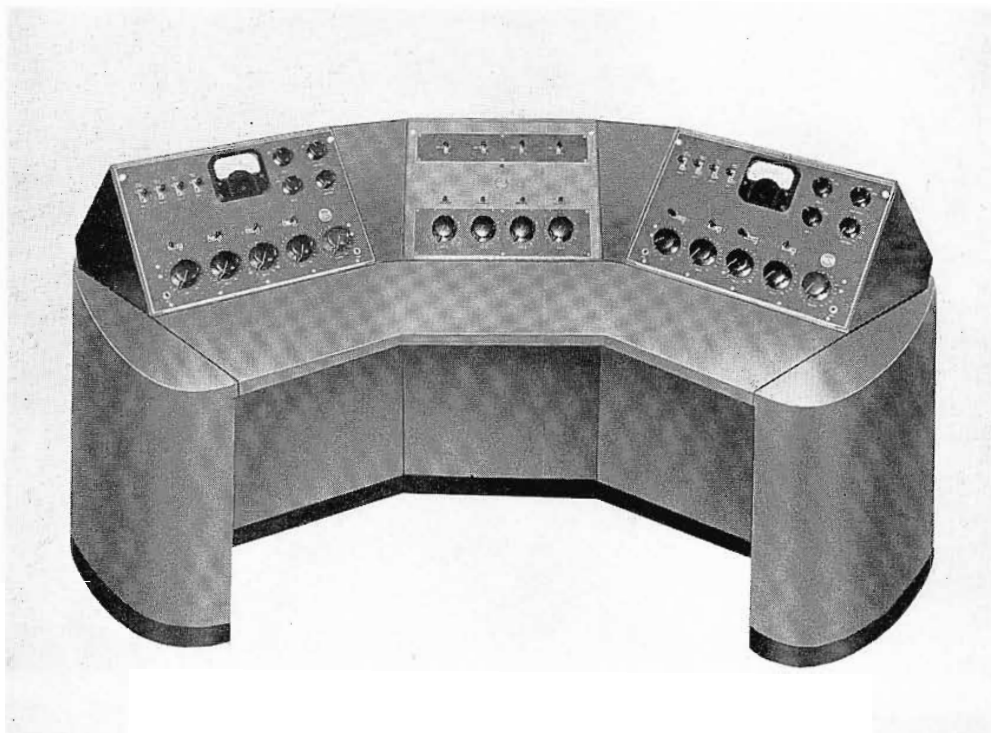
FIG. 6. A deluxe "U" arrangement of two BC-5A's flanking a BCM-1A Auxiliary mixer lends a "custom touch" with considerable versatility. Connections for this arrangement are handled in a similar manner to that described for BC-2B (Fig. 5).
