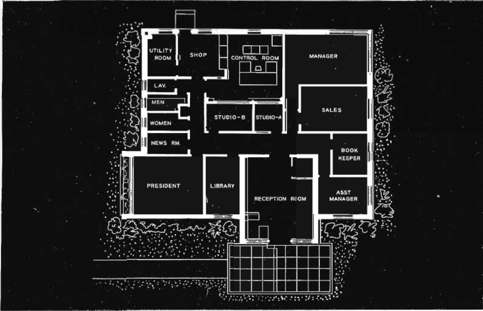
FIG. 1. The new WDAS combined Studio/Transmitter building is functional as well as attractive. Interior arrangement is shown in floor plan at left. Details of construction are described in text.
