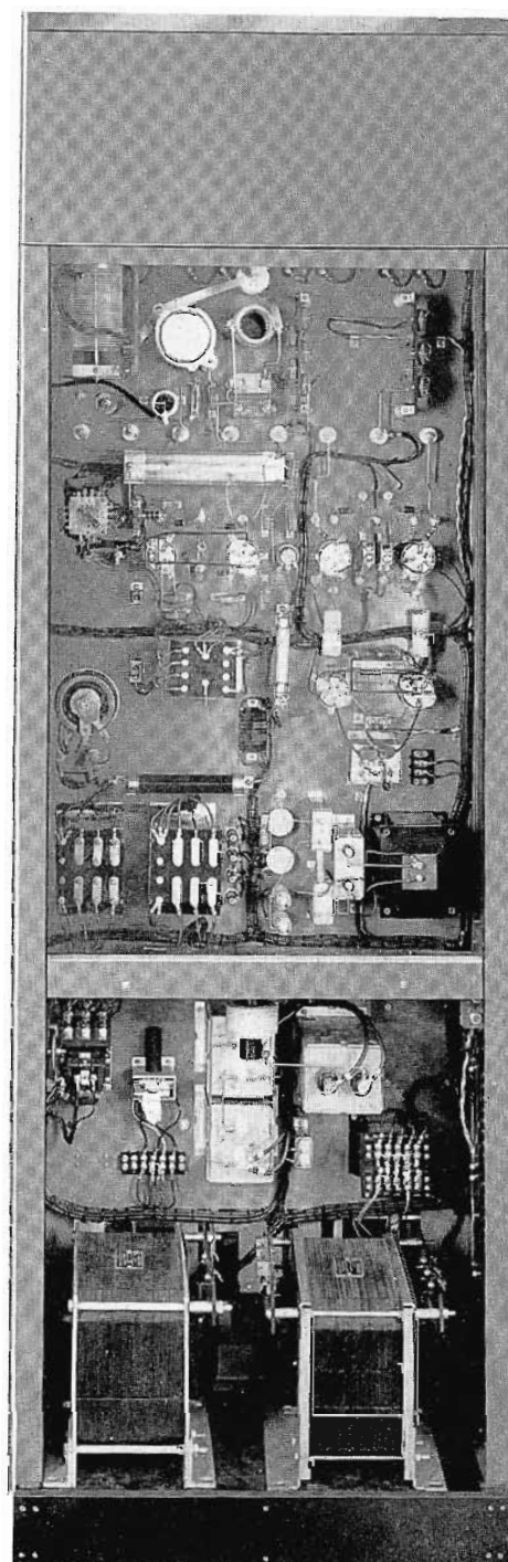
FIG. 5. Rear view of BTA-1MX/500MX, door removed, shows precise wiring and full accessibility to components.
