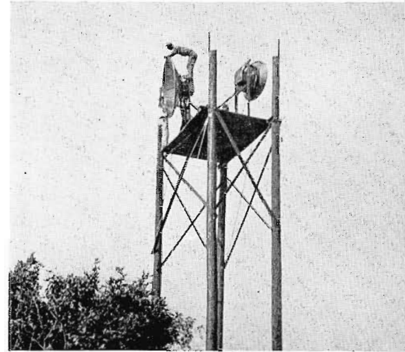
FIG. 12. Orienting parabolic reflector at Poor Mountain to line up with Dismal Peak.
