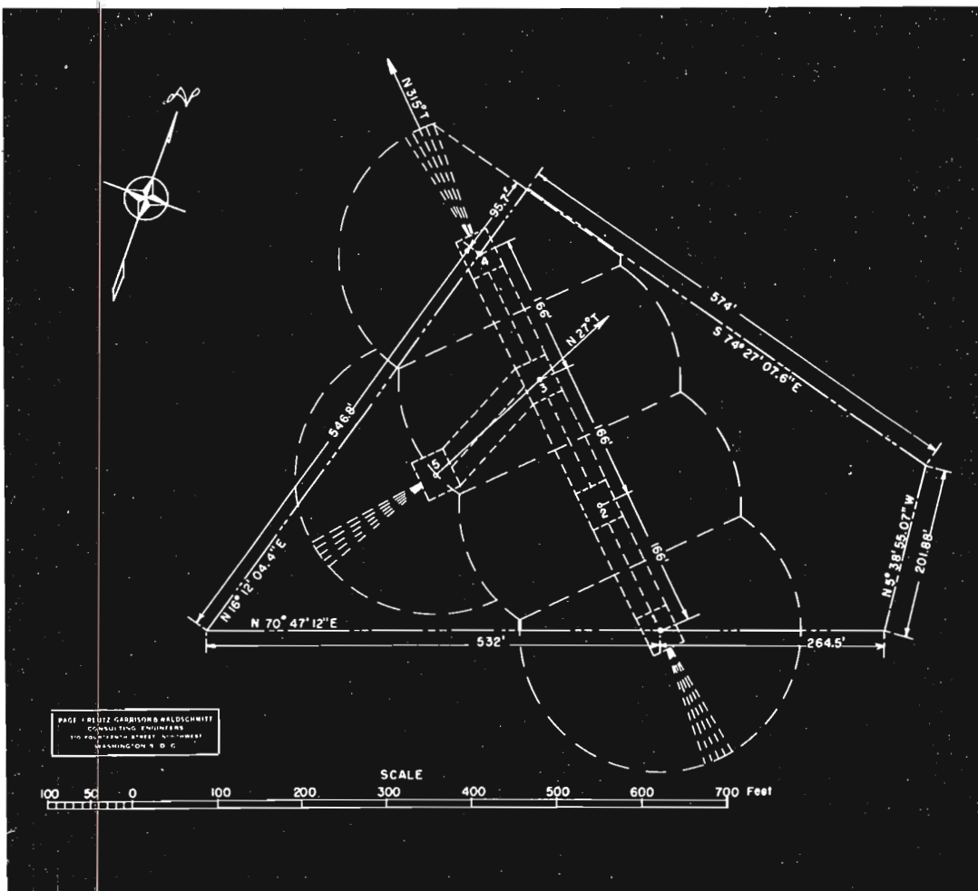
FIG. 11. Antenna locations and ground system. Towers Nos. 3 and 5 used for day operation—Nos. 1, 2, 3 and 4 used for night operation.
