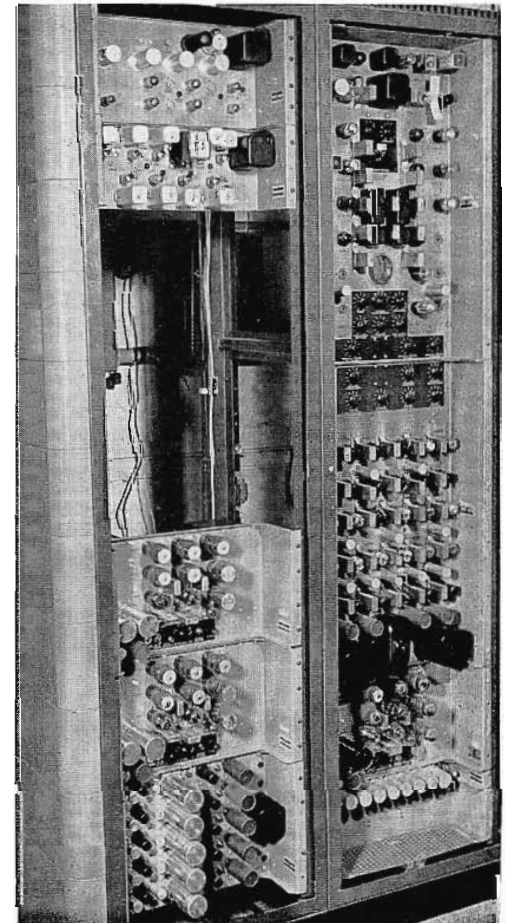
FIG. 8. Rack-mounted TG-1A synchronizing generator, power supplies and distribution amplifier.
