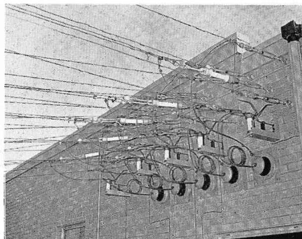
FIG. 6. Building dead-end termination of open wire line leading to five towers. Lightning protector horn-gaps are visible above each ground plate.
