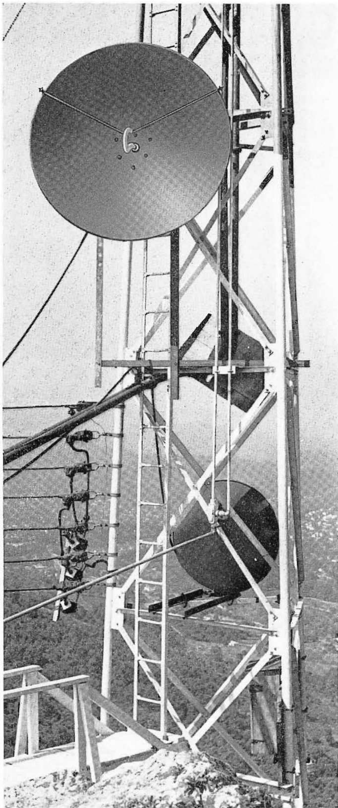
FIG. 1. Terminal of WHIS-TV Microwave system at East River Mountain, W. Virginia.
