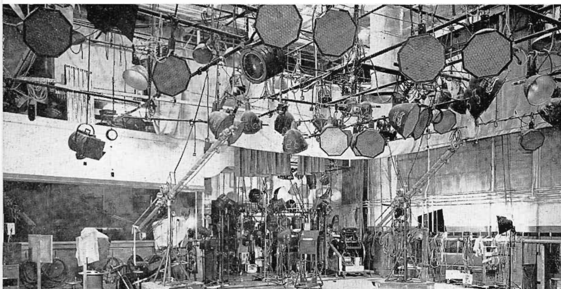
FIG. 1. (left). WNBQ's television Studio A as it looked just a few months ago. At the left rear is the control booth which was used for monochrome operation. To provide more space for color studio operation this booth is being removed. Lighting and air conditioning systems are being modernized and the studio generally refurbished.
