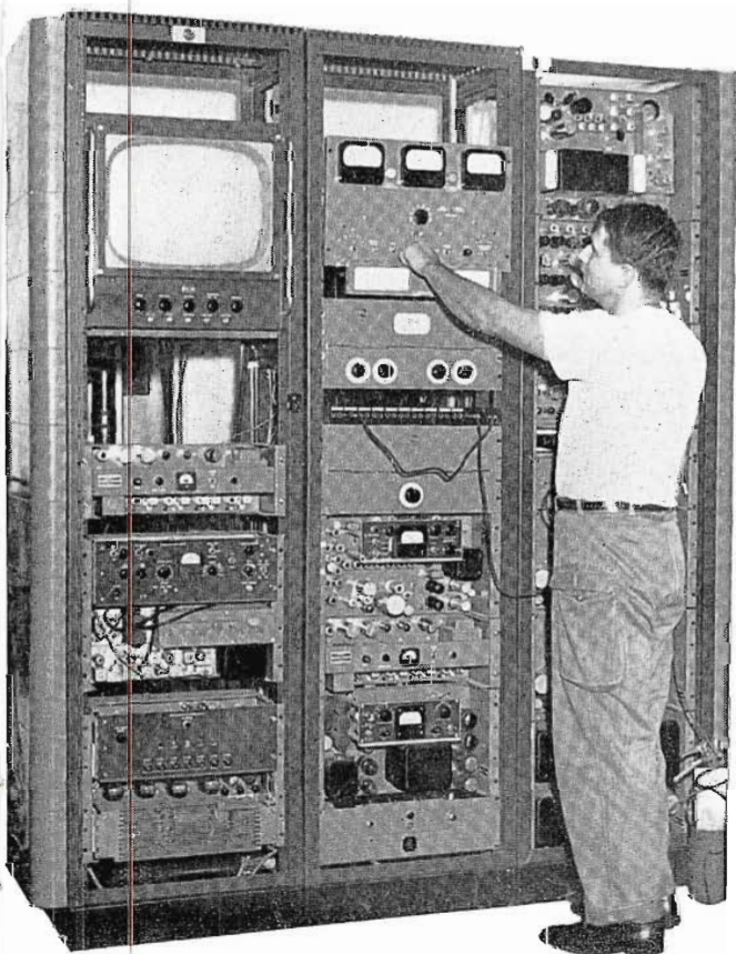
FIG. 11. Racks in transmitter room contain microwave terminations, frequency monitor, power supplies and other equipment.
