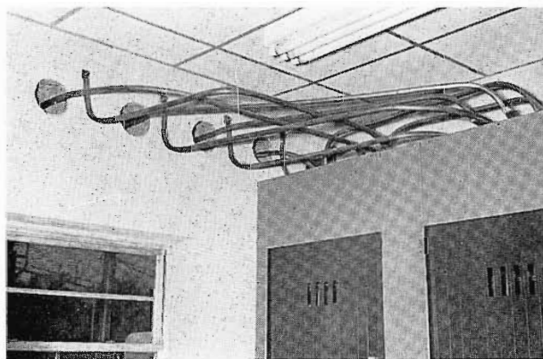
FIG. 5. View showing transmission line feed to feed-thru insulators. Lines fastened directly to wall connect through to ground plates on outer wall.
