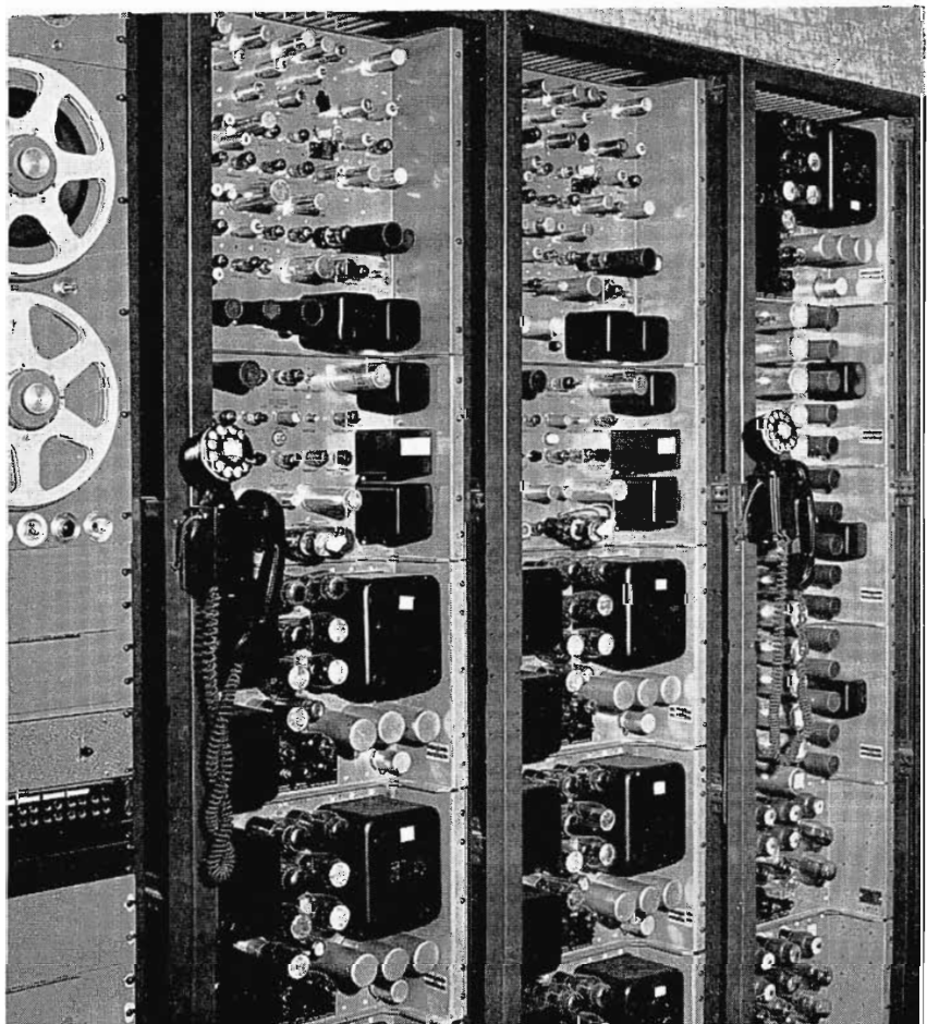
The center two cabinet racks contain auxiliary and power requirements. Each rack contains (top to bottom) the vidicon control chassis, the vidicon deflection chassis and two WP-33B power supplies necessary for operation of the film chain. The other WP-33B power supplies are used for operation of other equipments.
