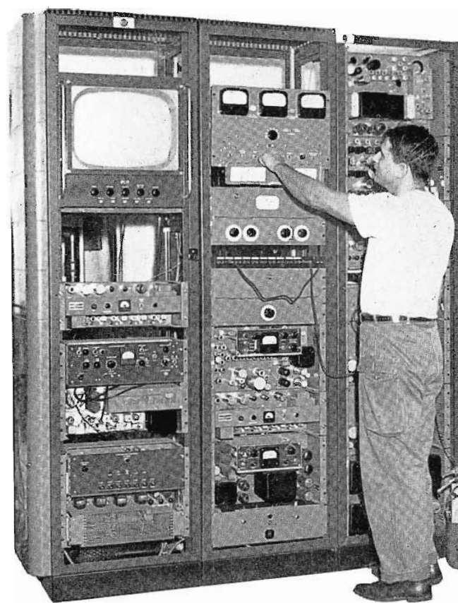
FIG. 18. Microwave equipment in station transmitter room. Left rack: microwave from Roanoke (NBC). Center rack: microwave from Bluefield (STL). Right rack: power supplies.
