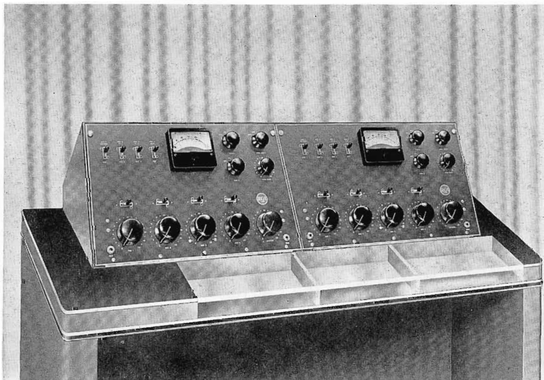
FIG. 4. Expandability of BC-5A facilities is simple and effective by pairing . . . provides dual channel operation.
