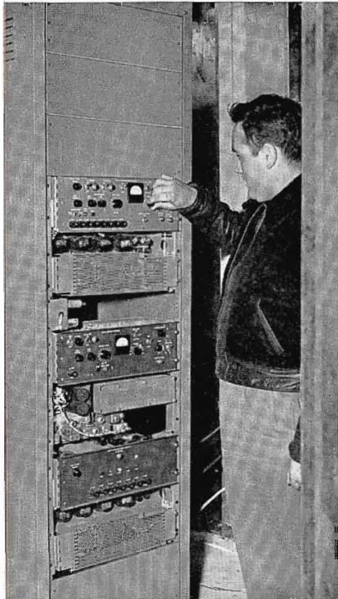
FIG. 13. Engineer Oliver Lienhard adjusting microwave equipment in relay station building at Poor Mountain.
