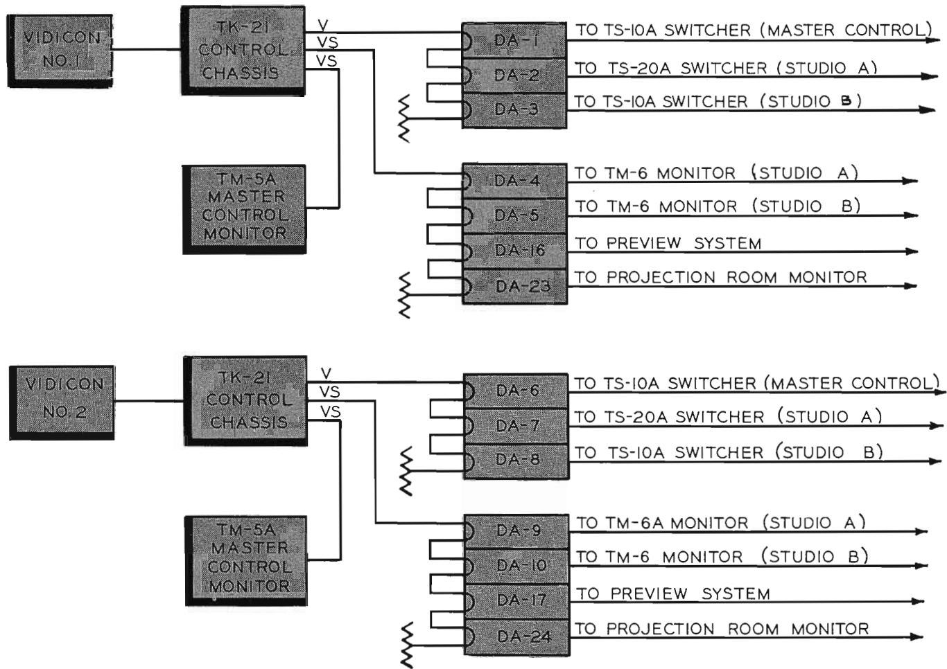
Block diagram showing video distribution of the two WAAM-TV Vidicon film chains.
