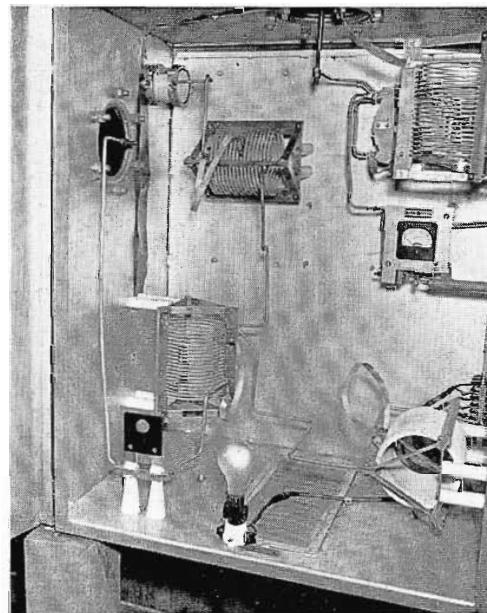
FIG. 15. Interior of LTU. 100 watt bulb keeps down dampness—provides light for reading meter through the door porthole.
