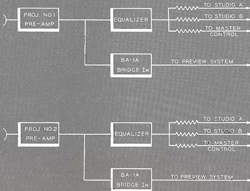
Block diagram showing distribution of audio from the two TP-16 projectors associated with the vidicon film chains.
