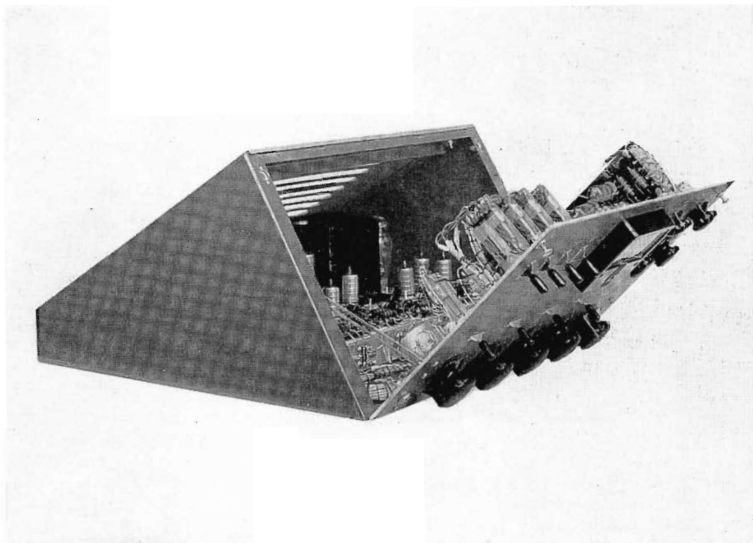
FIG. 3. View showing BC-5A interior by opening front panel. Printed wiring boards are mounted on horizontal chassis. Another is visible at upper right corner inside front panel.
