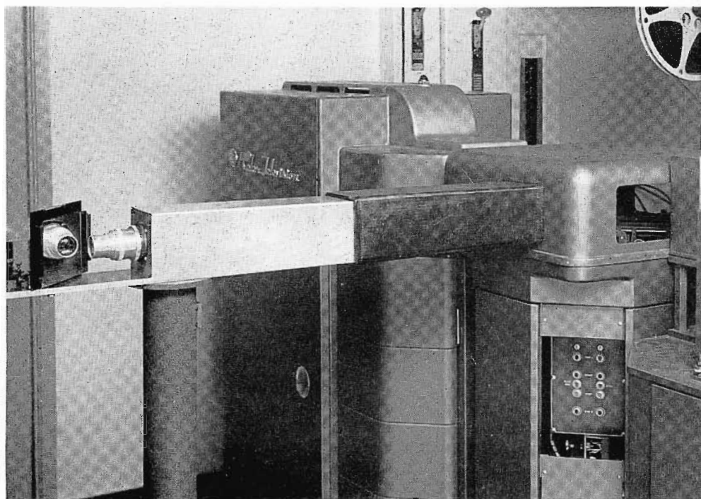
FIG. 4. Standard 3-V Color film chain with optical system for feeding live color commercials. Light shield and dust covers are in position.
