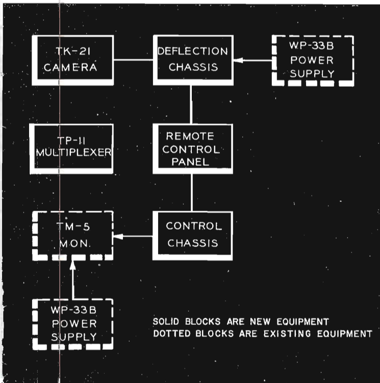
Functional block diagram of WAAM-TV's vidicon camera equipment. Equipments show in solid lines were the only new items required for conversion of each film chain. In addition to the existing equipment shown in dotted blocks, the station was also able to use their original projectors and console housings.
