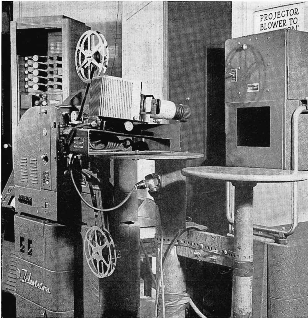
FIG. 7. Film facilities include a TK-20A film camera and film camera control. The projector is an RCA TP-16 16-mm film projector.
