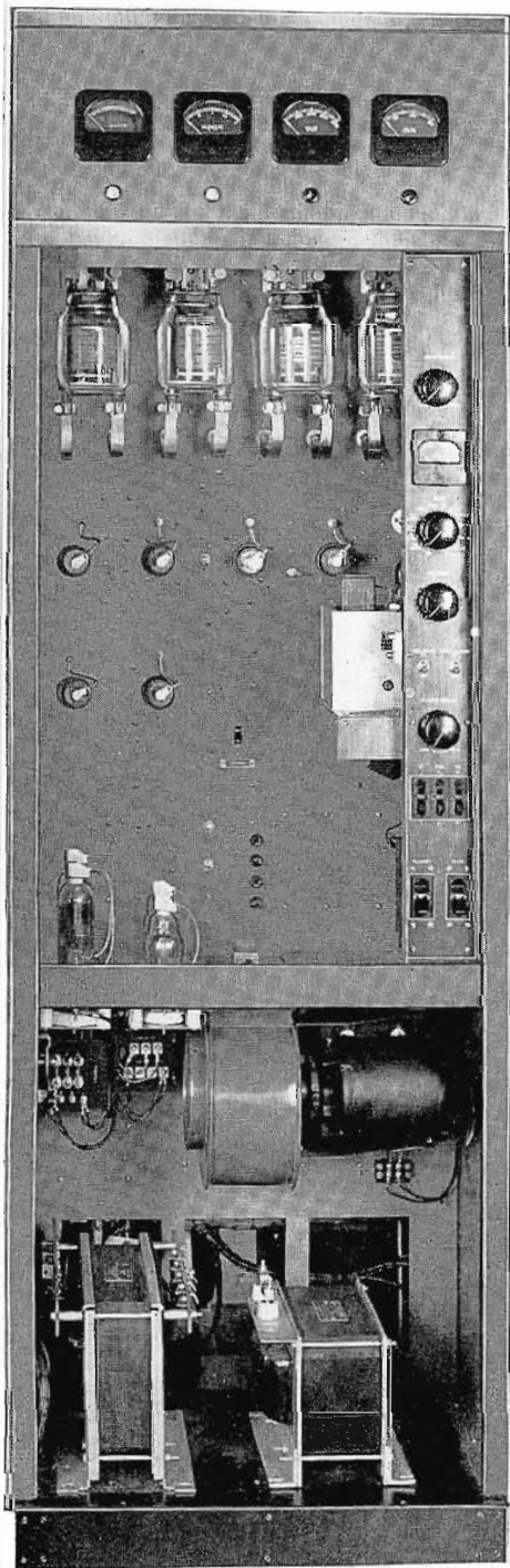
FIG. 4. Front view of BTA-1MX/500MX, doors removed, shows overall simplicity of component arrangement.
