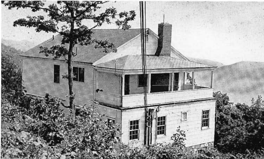
FIG. 9. Transmitter is housed in building which also provides living quarters for transmitter engineer and family on second floor.
