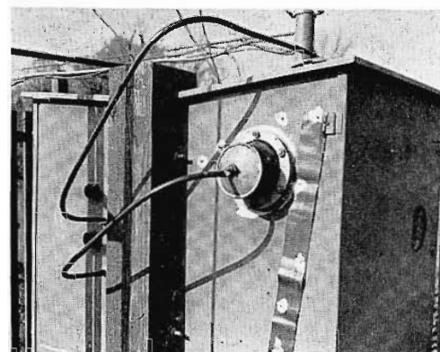
FIG. 14. Tuning houses back-to-back for day-to-night pattern tower.
