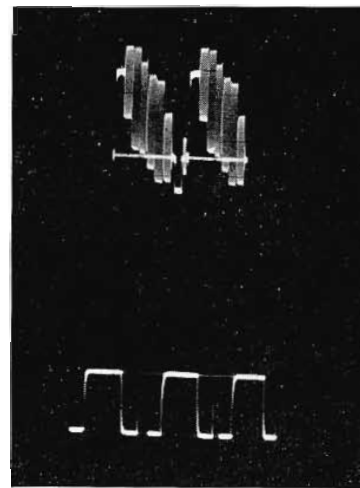
FIG. 15. Above: Colorplexer output signal for a color bar test pattern displayed at half-horizontal frequencies. Below: Typical display showing calibrating square wave with electronic calibration lines superimposed in the background.
