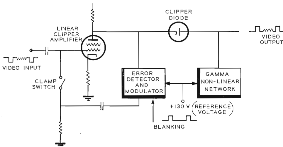
FIG. 7. A block diagram of feedback clamp circuit.
