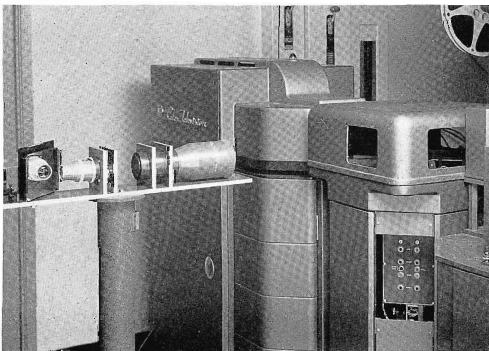
FIG. 5. Lens system—with covers removed—for adding live action color commercials using RCA 3-V film chain.
