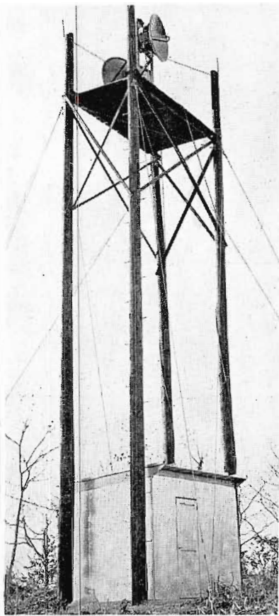
FIG. 3. Microwave relay station, Poor Mountain, Virginia.
