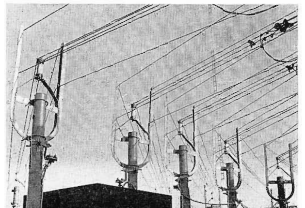
FIG. 8. Pole-mounted bayonet insulators support the open-wire transmission line runs. Although not visible these poles also support sampling lines.
