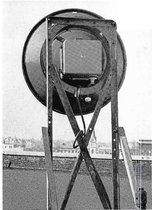
FIG. 15. Rear view of roof top microwave installation at Roanoke.
