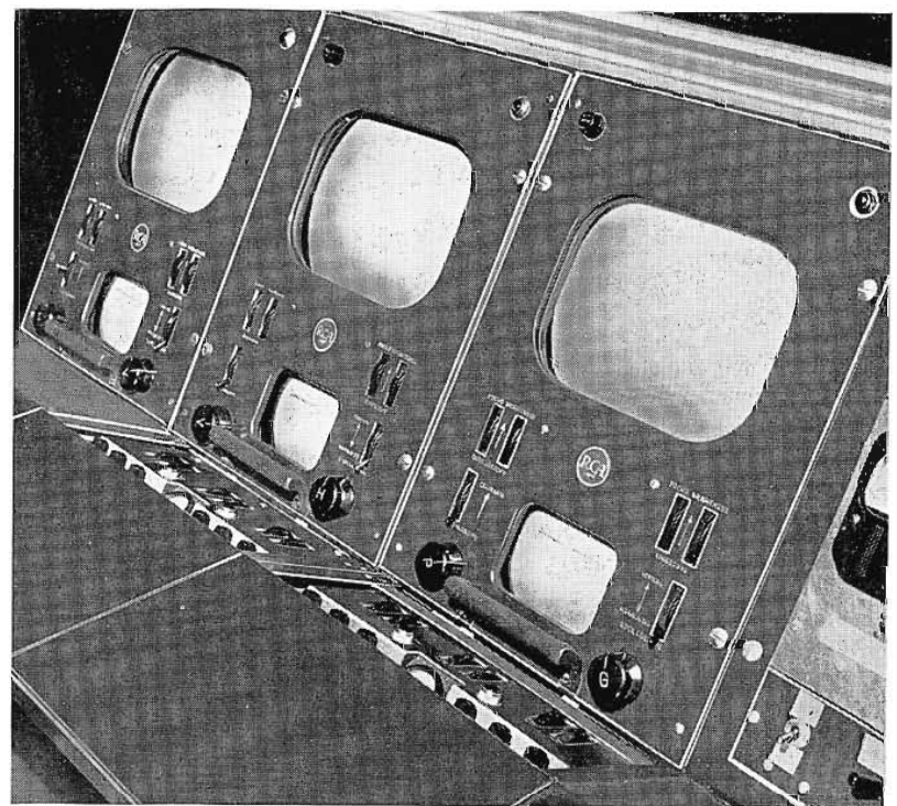
Closeup of the vidicon master monitors in their control housings. Use of existing equipment greatly simplified the installation. No changes in arrangement were required in the master control room. Vidicon remote control panels were substituted for the control panels of the iconoscope cameras. Auxiliary iconoscope equipment previously mounted in the base of the console housings was removed.
