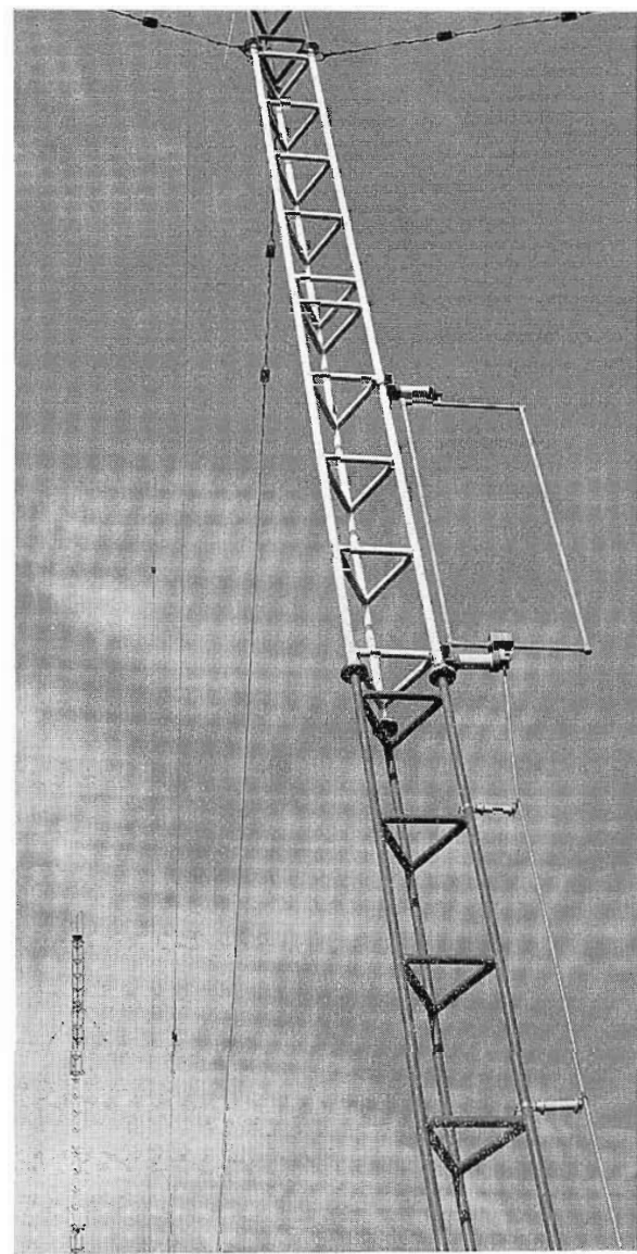
FIG. 10. Close-up of one of five Stainless guyed towers showing sampling loop and sampling line insulated from tower. Tower heights—148 feet—do not require lighting.
