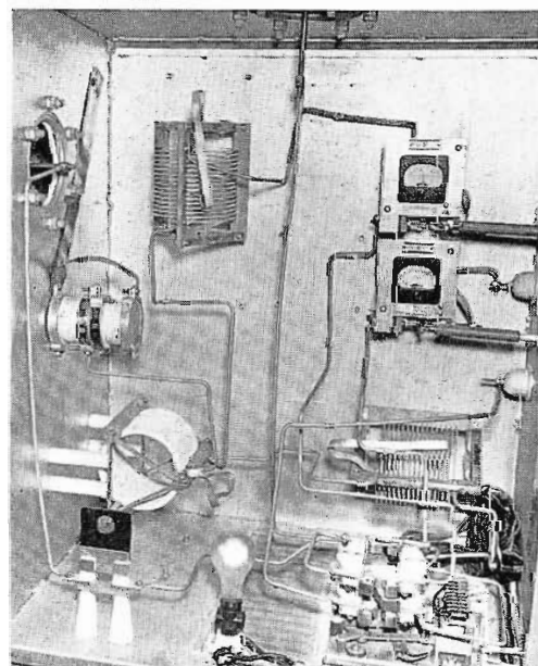
FIG. 13. Line terminating unit interior showing switch for day/night patterns. Two meters are for day current and night current measurement.
