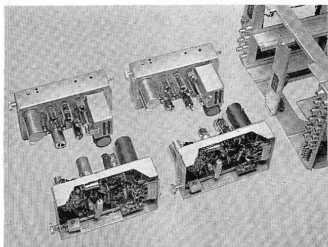
FIG. 4. The basic circuit elements of the processing amplifier are shown here—3 plug-in video amplifiers and a plug-in video section for an electronic switcher.
