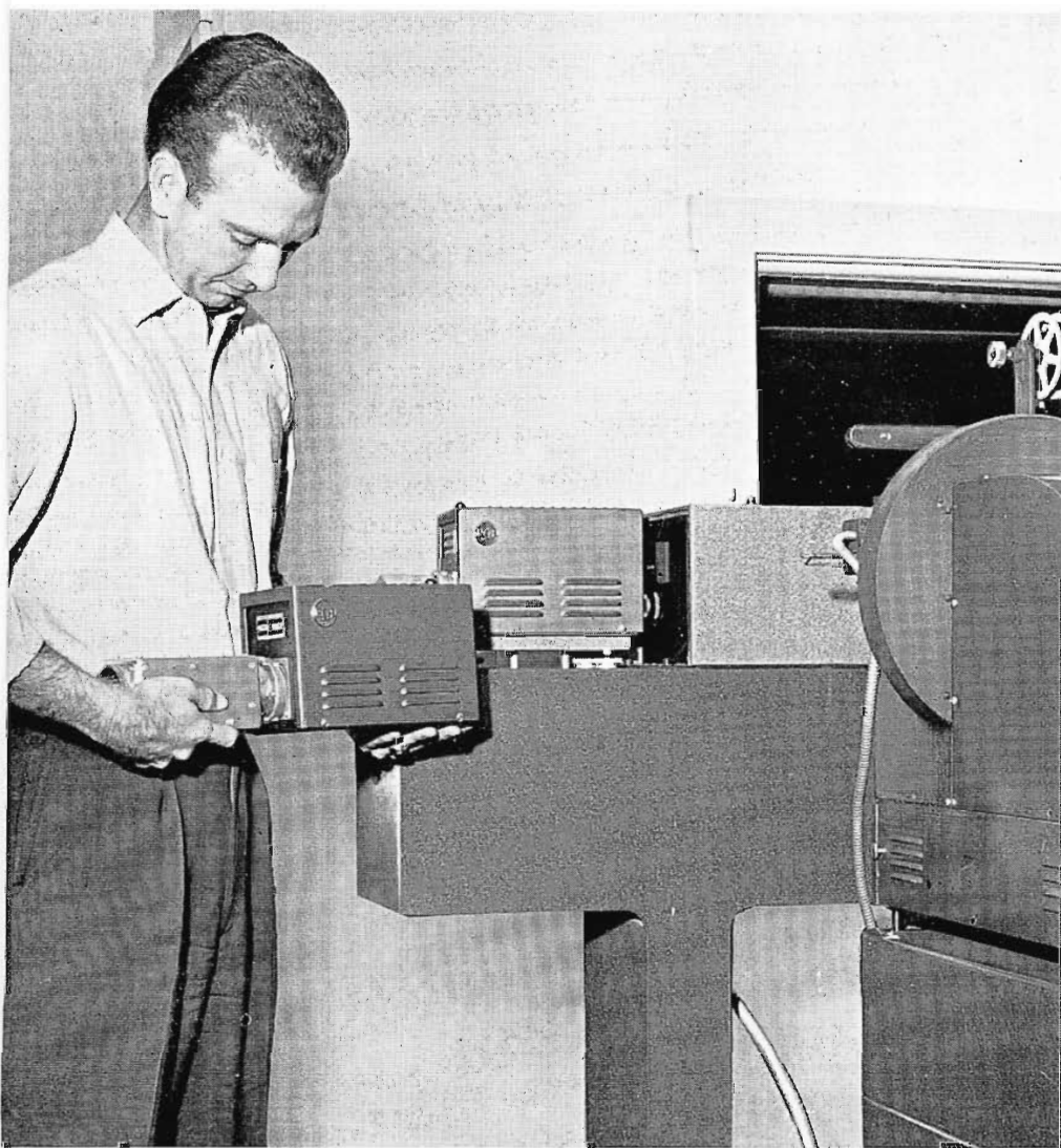
A complete vidicon camera chassis was ordered as a spare. This allows either of the film chains to be quickly returned to service in emergencies.
