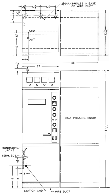
FIG. 1. The BTA-1MX/500MX with all the virtues of its predecessor (BTA-1M) and more. Has bi-level modulation, full enclosure doors for excellent cabinet shielding, improved remote control adaptability. Occupies only 6.2 square feet of floor space.
