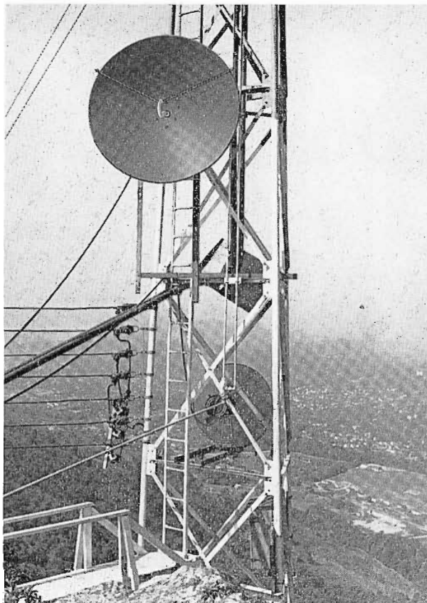
FIG. 12. Transmitter tower showing microwave dish of 3-hop system (at top) and rear of STL dish (beneath).
