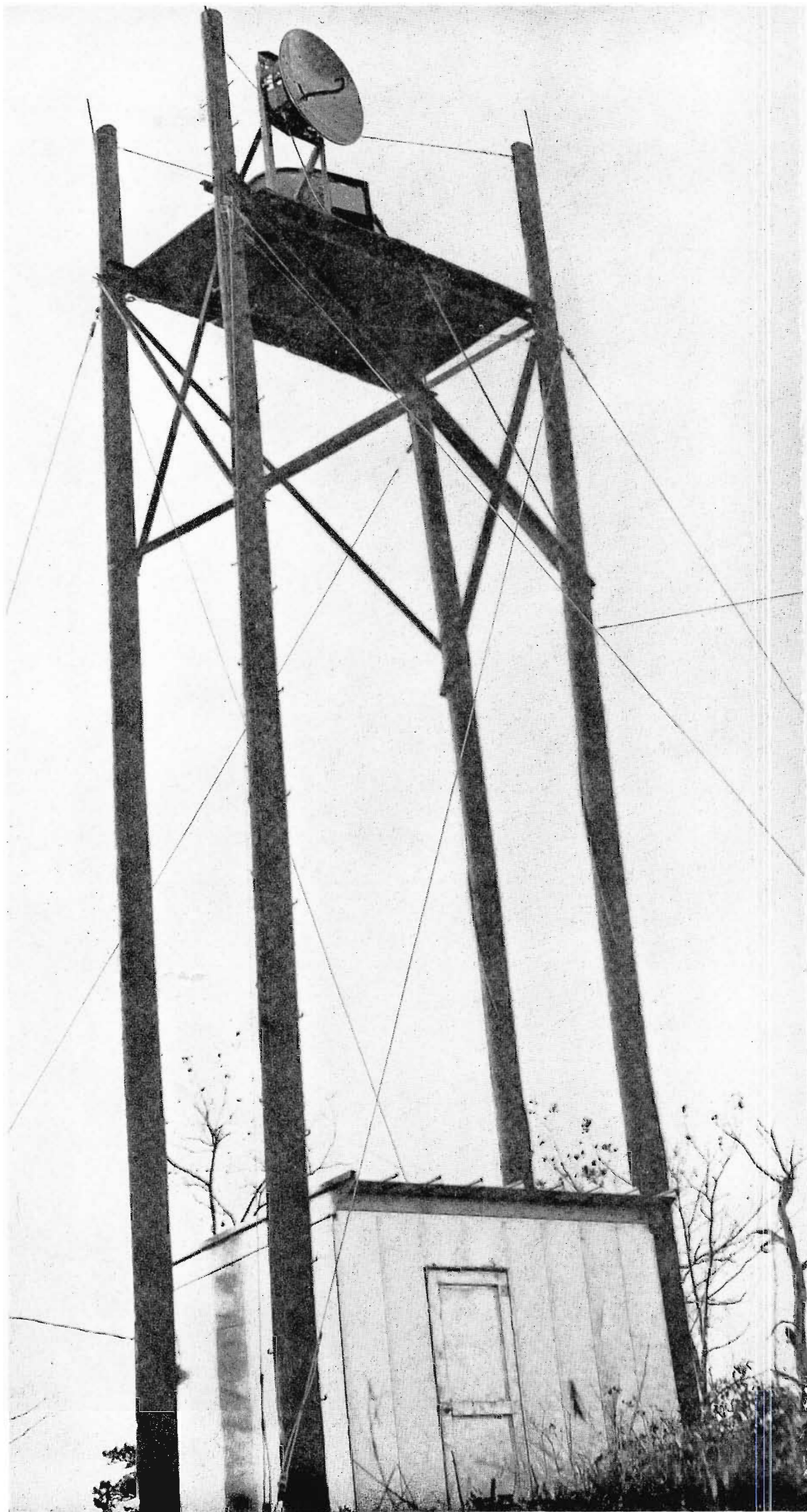
FIG. 9. Construction of typical microwave relay tower using 4 telephone poles for supporting 6 foot dishes and head end equipments for transmitting and receiving.
