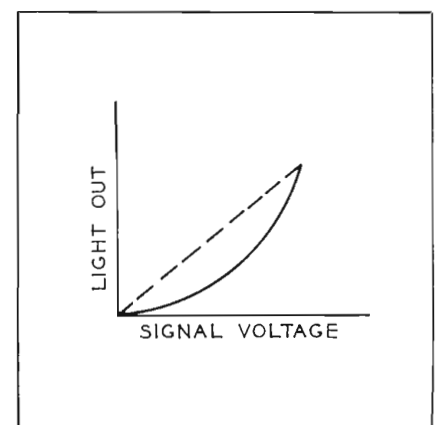
FIG. 8. Transfer curve of an average kinescope.
