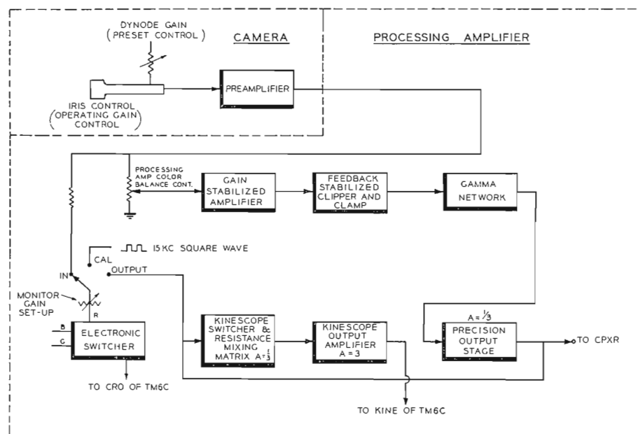
FIG. 5. A block diagram showing the gain control function incorporated in the processing amplifier.
