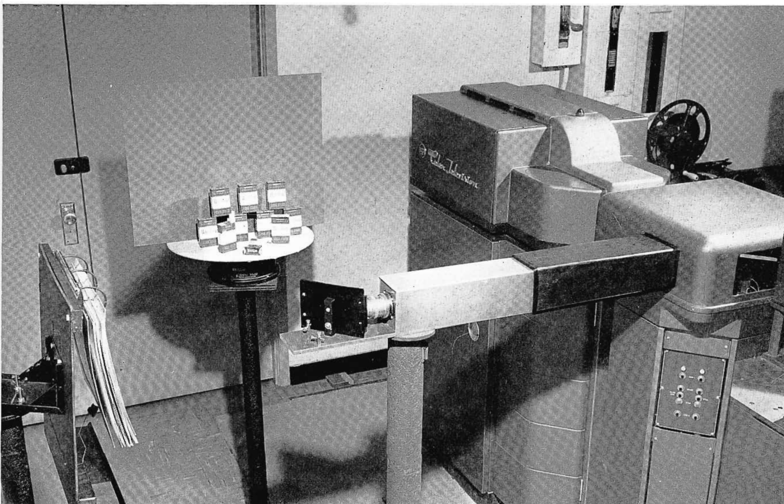
FIG. 1. Lens system added to RCA TK-26A 3-V Color Film Chain for pickup of live color commercials and color opaques.
