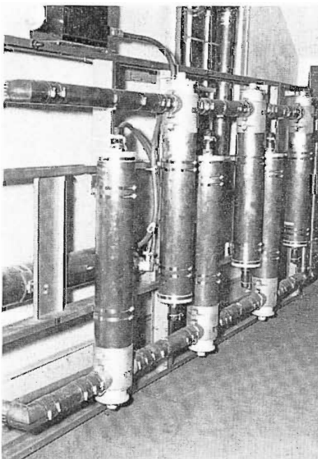
FIG. 13. Vestigial side band filter is installed in corridor adjacent to transmitter room.
