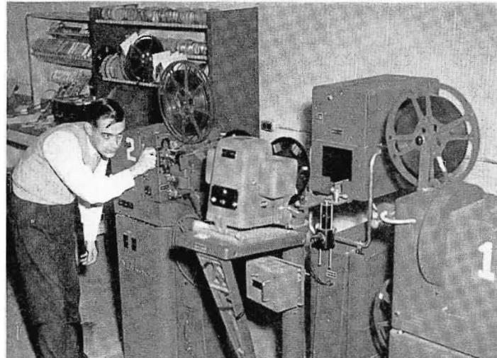
FIG. 6. The film room is equipped with two RCA 16mm TV film projectors, 35mm slide projector and RCA film camera.
